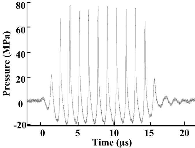
Fig. 2. Acoustic pressure waveform of a 10-cycle (14- \mu s) histotripsy pulse in water at the transducer focus (P R = 21 MPa, P C = 76 MPa).
