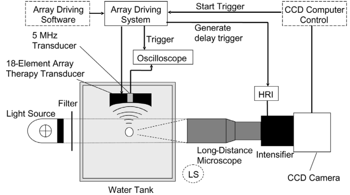
Fig. 1. Schematic drawing of experimental setup for high speed imaging and acoustic backscatter recording. The light source position shown was for bubble shadowgraph acquisition. For whole bubble cloud imaging with forward lighting, the long-distance microscope was replaced by lenses described in the methods section and the light source was moved to the position labeled as “LS” (dashed circle).
