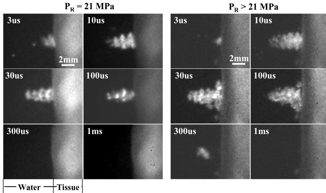
Fig. 8. Images of bubble clouds generated by a 10-cycle (14- \mu s) pulse at P_R of 21 MPa (left) and > 21 MPa (right) at a tissue-water interface. Each image was taken at a specific time delay (labeled) after the arrival of the histotripsy pulse at the transducer focus (i.e., tissue surface). The bubble cloud was larger and longer in duration at higher P_R .
