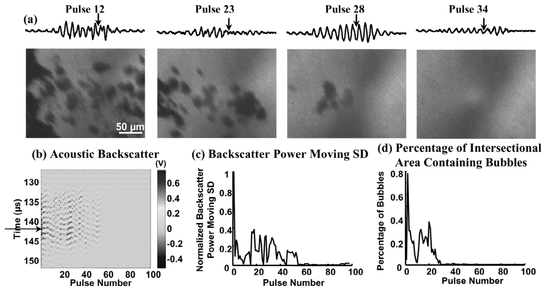
Fig. 6. (a) Waveforms of the range-gated acoustic backscatter signals (top) and the corresponding bubble shadowgraphs (bottom) produced inside a gelatin phantom. (b) Acoustic backscatter signals, (c) backscatter power moving SD, and (d) percentage of intersectional area containing bubbles displayed in the same format as Fig. 5(b)–(d). Arrows on the acoustic backscatter trace in (a) and acoustic backscatter fast-time and slow-time image in (b) indicate when the optical image was taken. The disappearance of bubbles and the extinction of the variable acoustic backscatter were observed.
