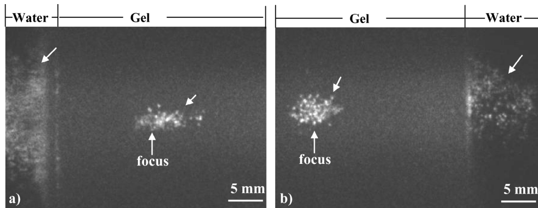
Fig. 8. Images of bubble clouds generated by a 10-cycle (14- \mu s) pulse at P_R of 21 MPa (left) and > 21 MPa (right) at a tissue-water interface. Each image was taken at a specific time delay (labeled) after the arrival of the histotripsy pulse at the transducer focus (i.e., tissue surface). The bubble cloud was larger and longer in duration at higher P_R .
